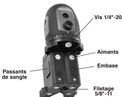
Figure 6 – Embase
