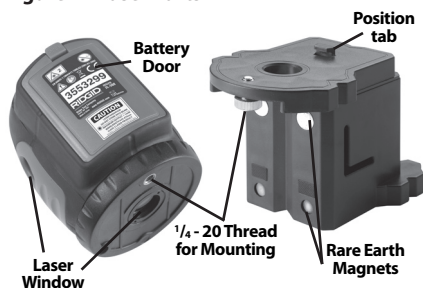
Figure 3 - Laser Level Parts
