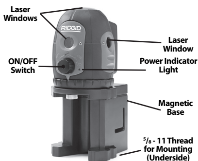
Figure 2 - Laser Parts
