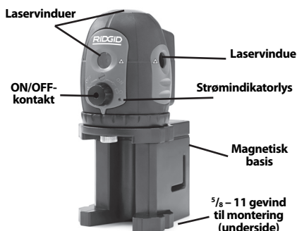
Figur 2 – laserdele
